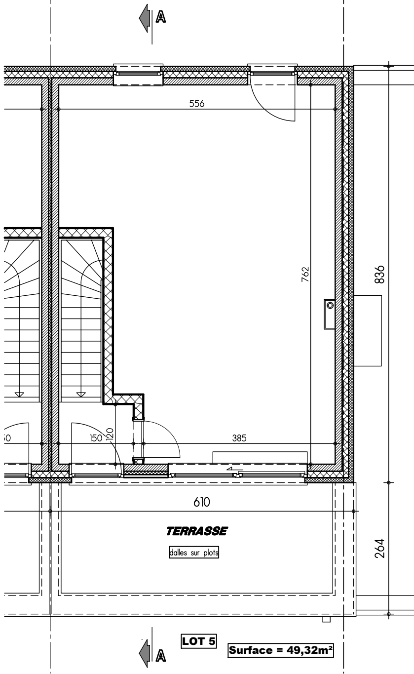
PLAN COMBLES
